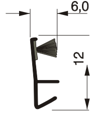
Ventilationsbürste Ventilating Brush
