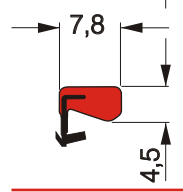
Stulpdichtung Seal for FRENCH windows
