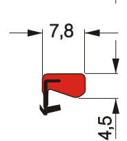
Stulpdichtung Seal for FRENCH windows
